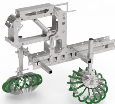
ROTOFILM ELEMENT
